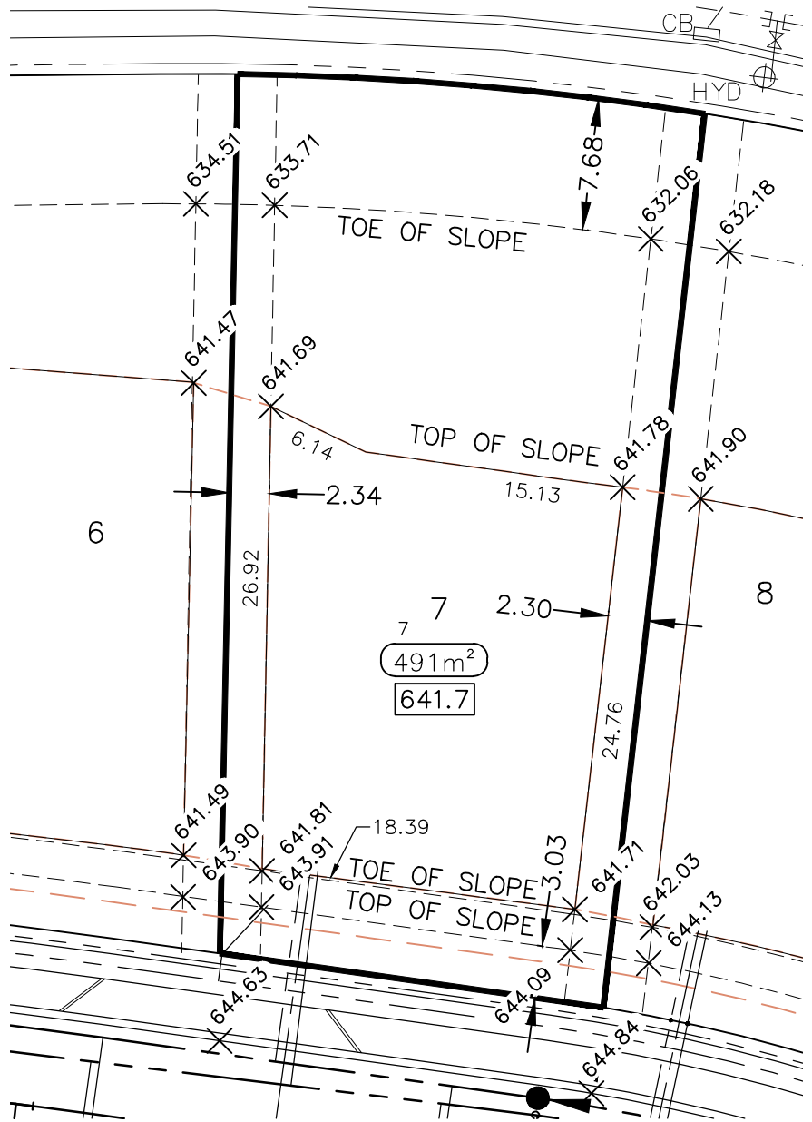
PLAN VIEW 1:400
