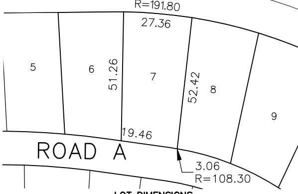
LOT DIMENSIONS 1:1500
