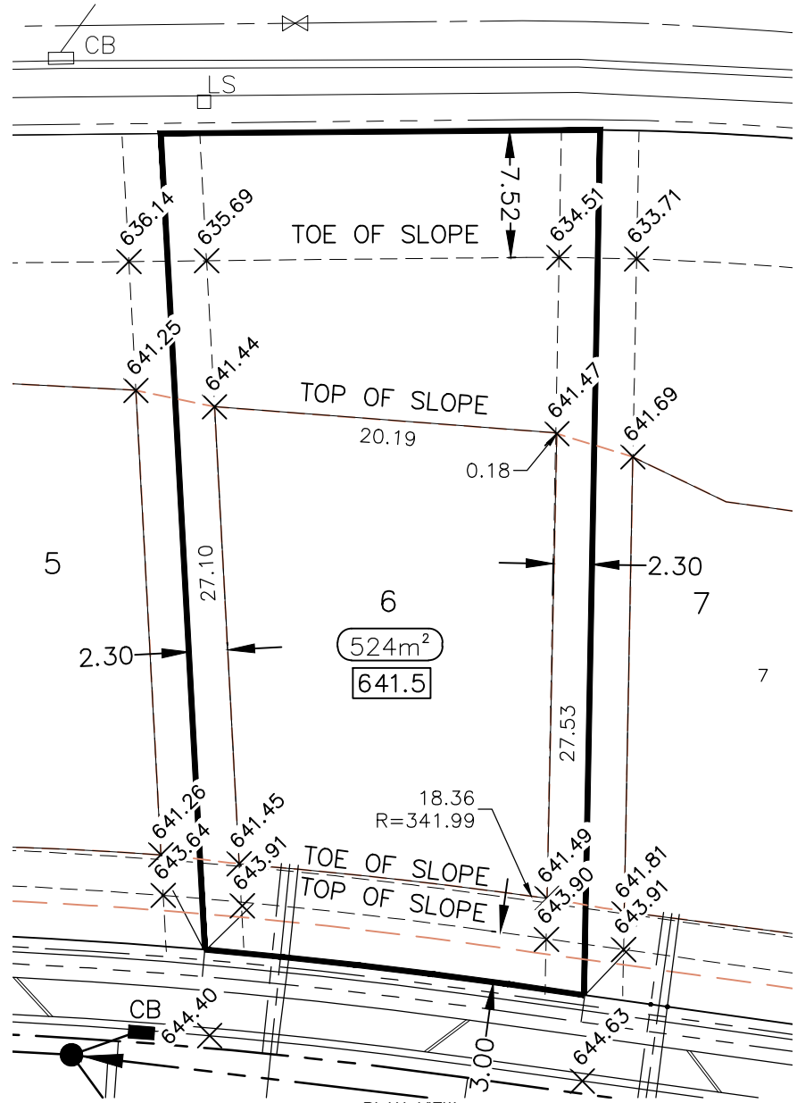
PLAN VIEW 1:400
