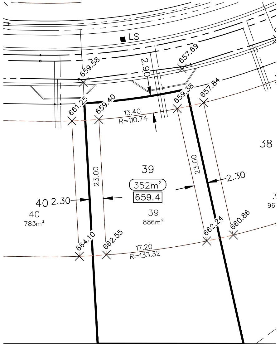
LOT DIMENSIONS 1:1500
