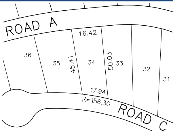
LOT DIMENSIONS 1:1500
