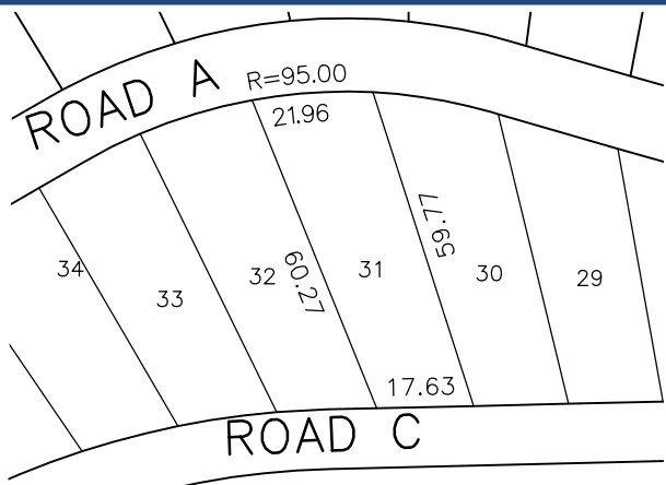
LOT DIMENSIONS 1:1500
