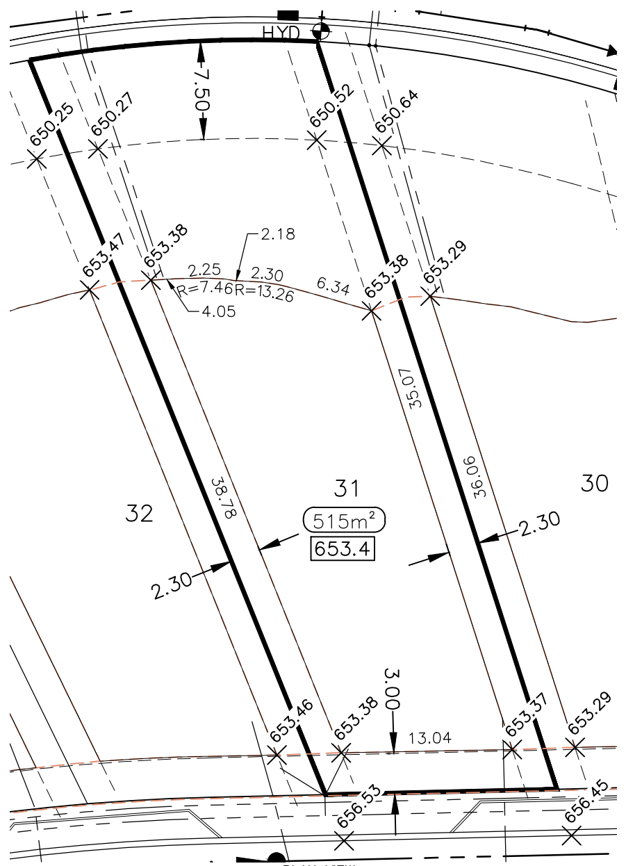
PLAN VIEW 1:400
