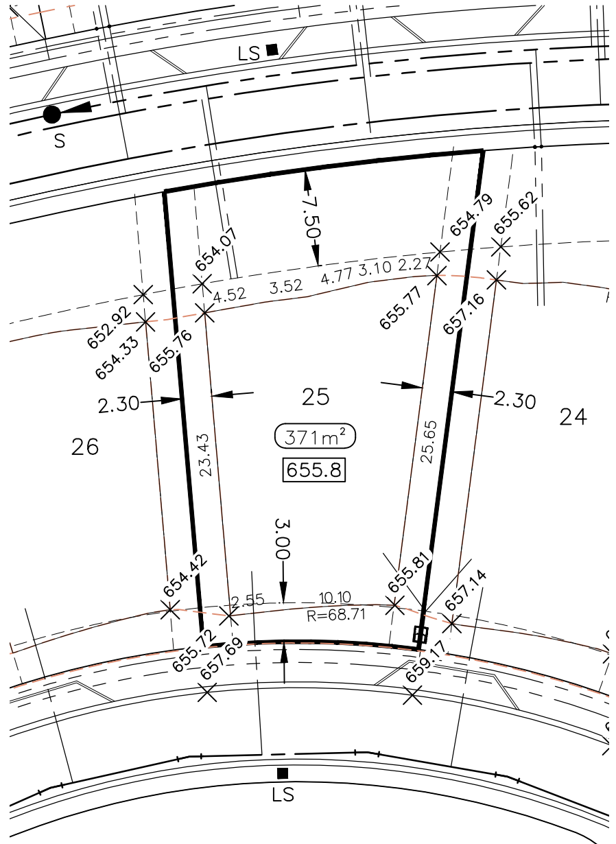
PLAN VIEW 1:400
