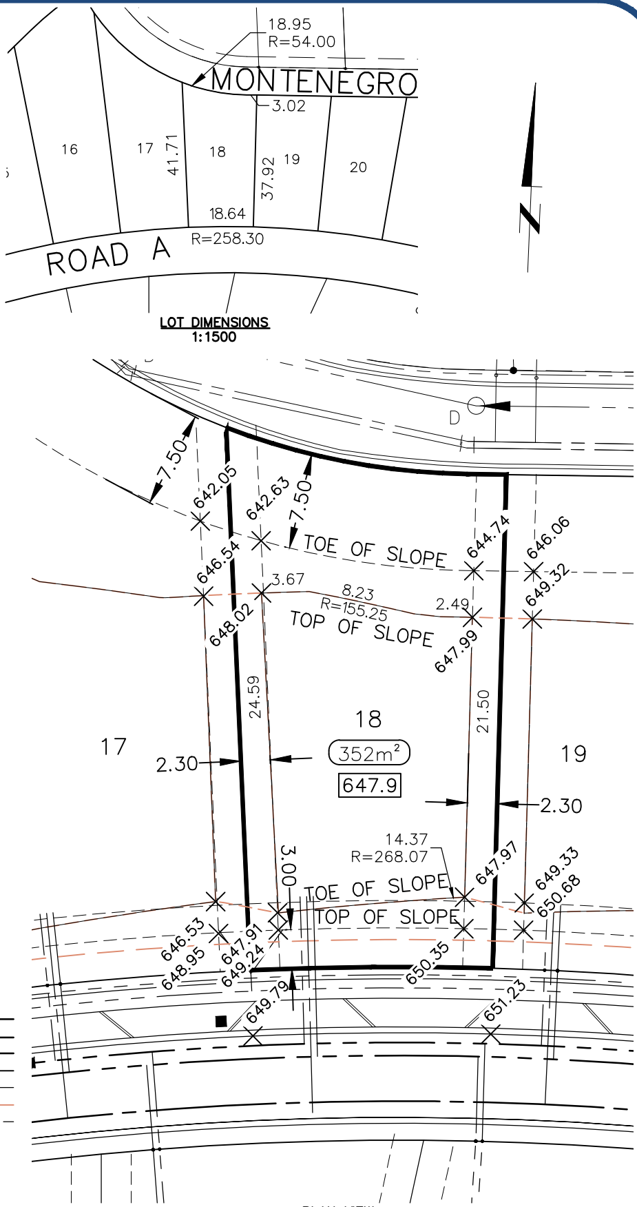
PLAN VIEW 1:400
