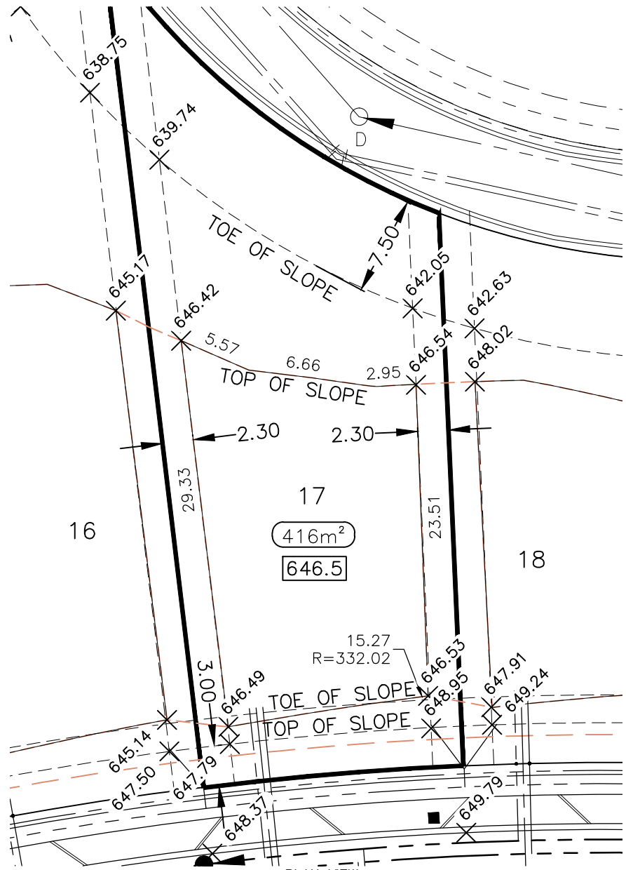
PLAN VIEW 1:400
